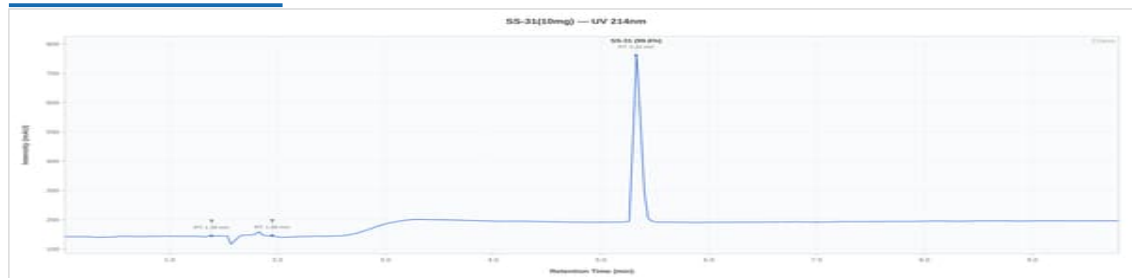
SS-31 10mg - SPP-0617-26: UV Chromatogram
