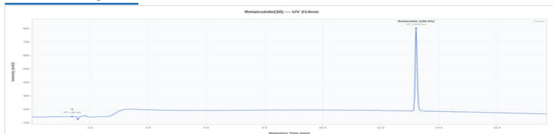
Retatrutide 30mg - SPP-0617-26: UV Chromatogram
