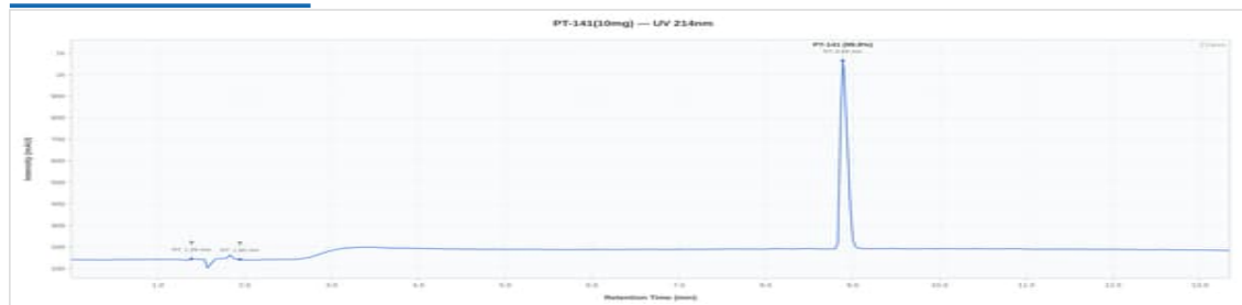
PT-141 10mg - SPP-0627-26: UV Chromatogram
