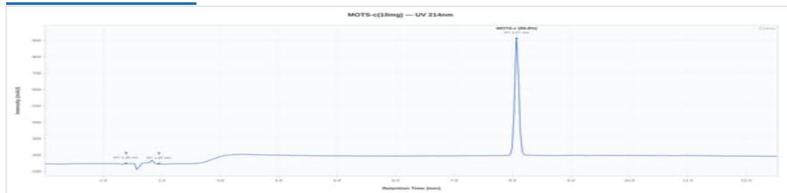
MOTS-C 10mg - SPP-0617-26: UV Chromatogram
