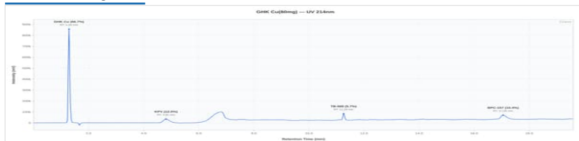
KLOW 80mg 80mg - 061826: UV Chromatogram
