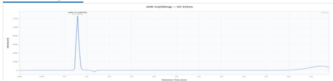
GHK-Cu 100mg - SPP-0617-26: UV Chromatogram
